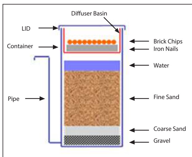
FIGURE 4: CROSS SECTION OF KAF
